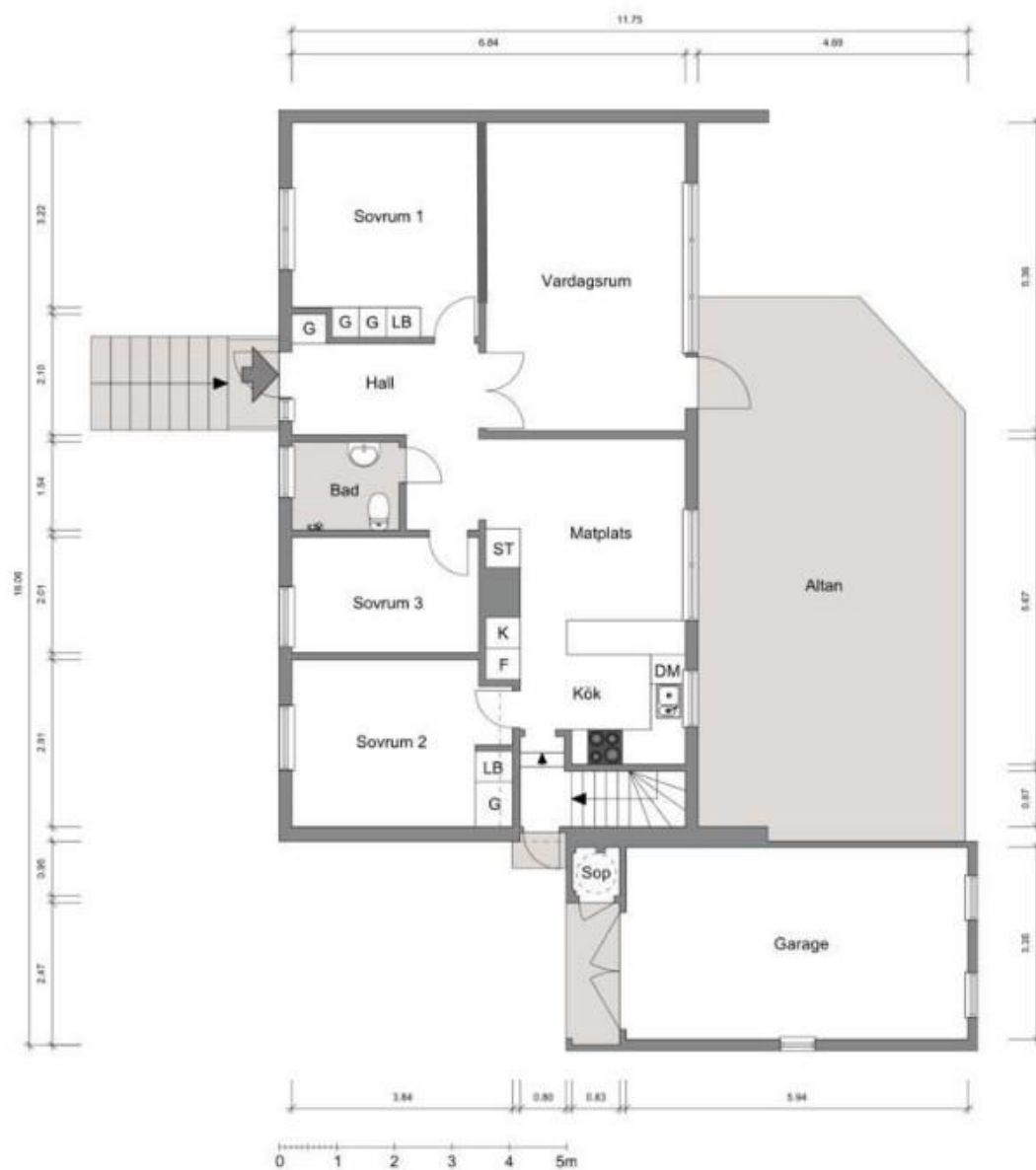
Bottenplan
