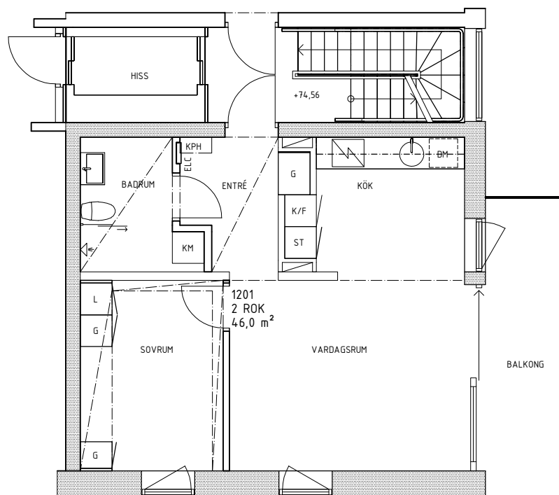
PLAN 2 TR
