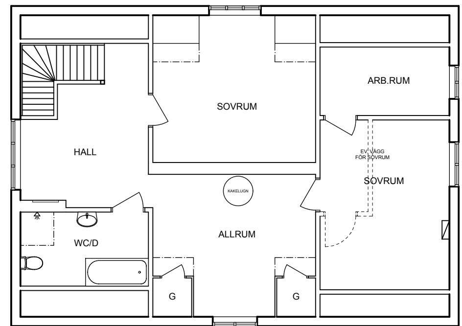
Plan 2
